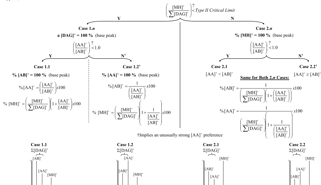
Scheme 2 Equations to calculate the relative abundances of the [MH]^+ ion and [DAG]^+ fragment ions for Type II TAGs using two Critical Ratios from APCI-MS data (Table 1), [MH]^+/\Sigma[DAG]^+ and [AA]^+/[AB]^+ . The Critical Limit for a Type II TAG is given in Fig. 6
